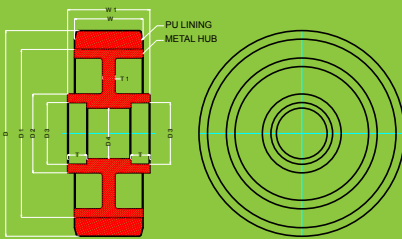
TROLLEY WHEEL
