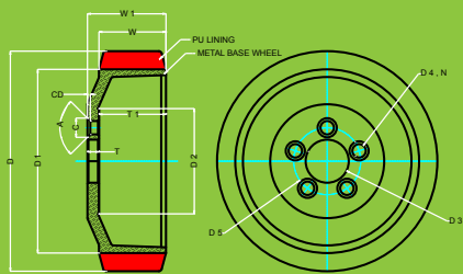
DRIVE WHEEL
